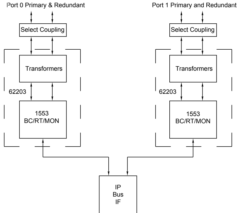
IP-1553 BLOCK DIAGRAM
