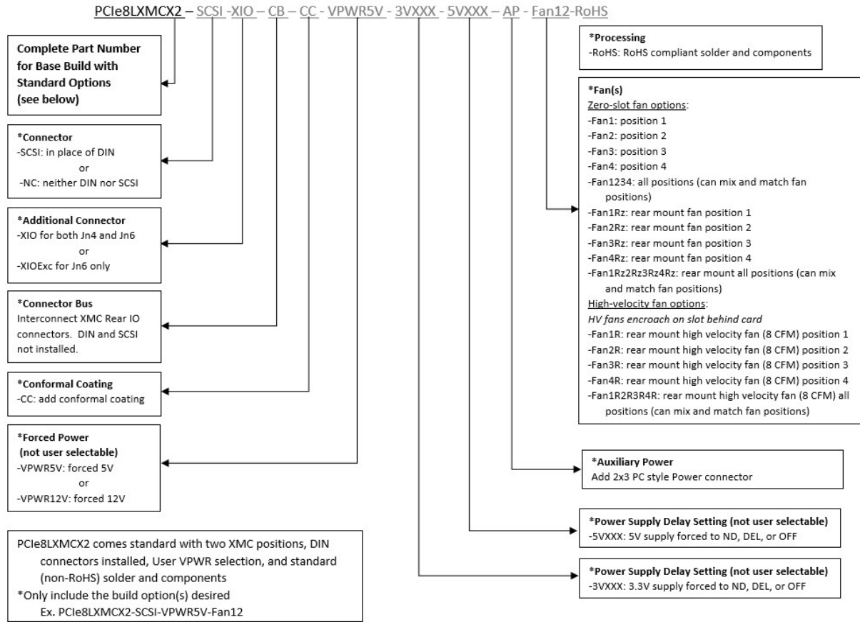
Figure 2: Ordering Options PCIe8LXMCX2
