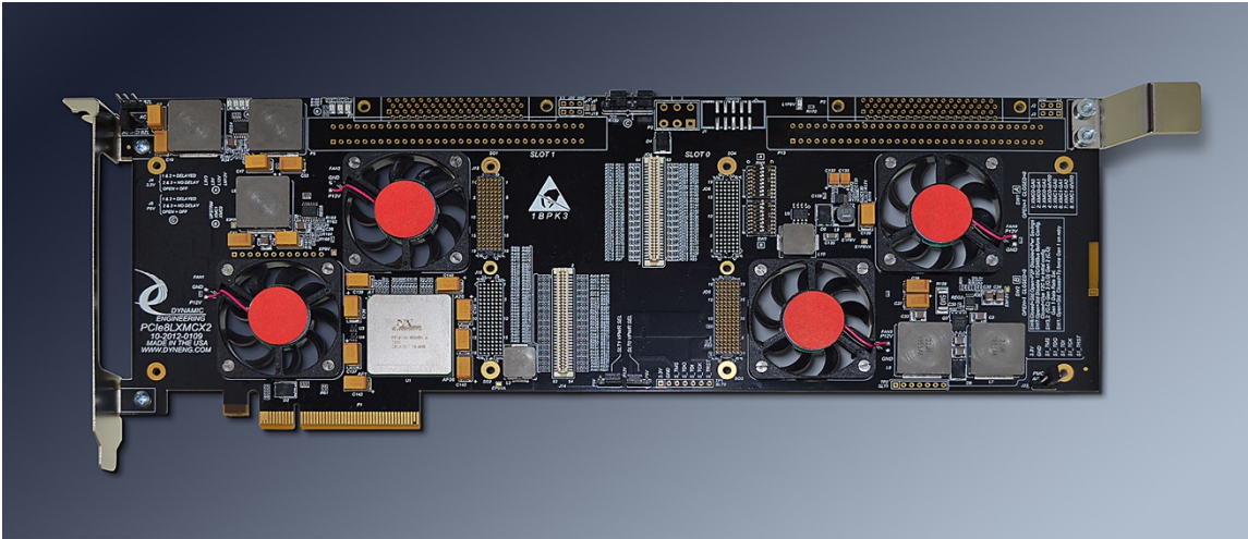
PCIe8LXMCX2 with CB option and Fans installed
