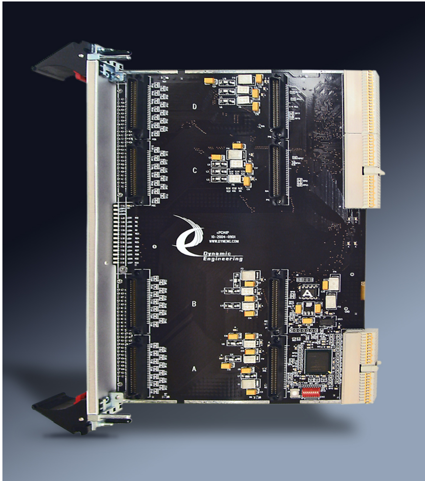
cPCI4IP Rear Panel IO version shown
