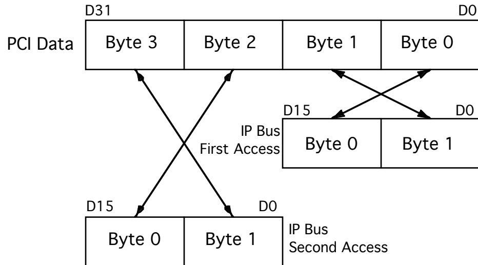
FIGURE 7 CPCI4IP 16 BIT BYTE SWAPPING
