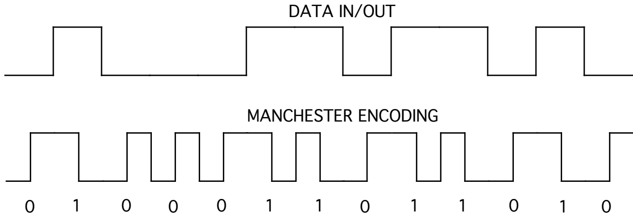
FIGURE 3 PMC BISERIAL III HW1 MANCHESTER TIMING DIAGRAM
