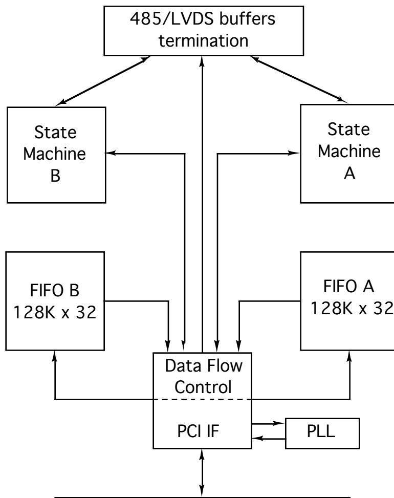
PMC BISERIAL-III BASE BLOCK DIAGRAM
