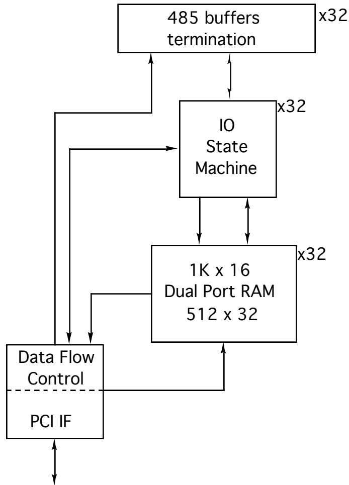
FIGURE 2 PMC BISERIAL-III-HW1 BLOCK DIAGRAM
